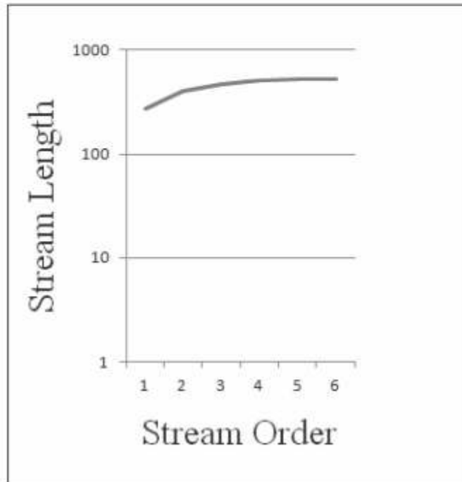
Figure 5 Stream Order VS Stream Length
