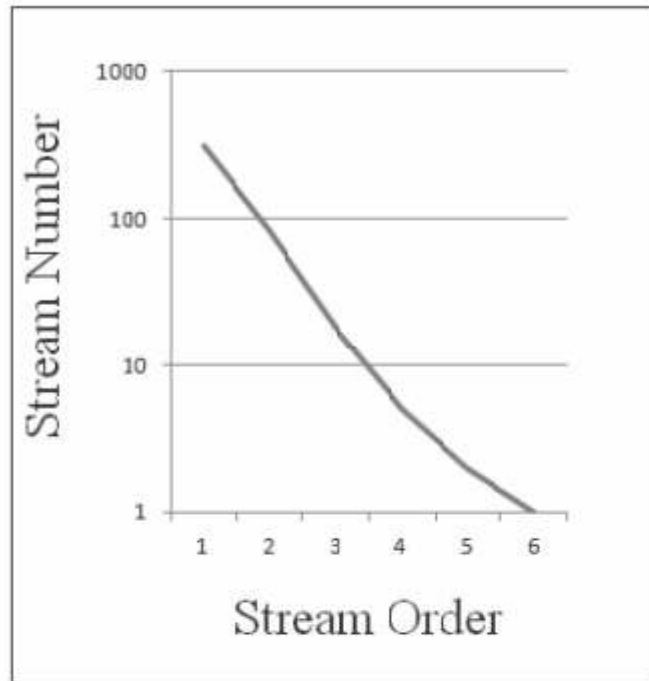
Figure 4 Stream order VS Stream Number
