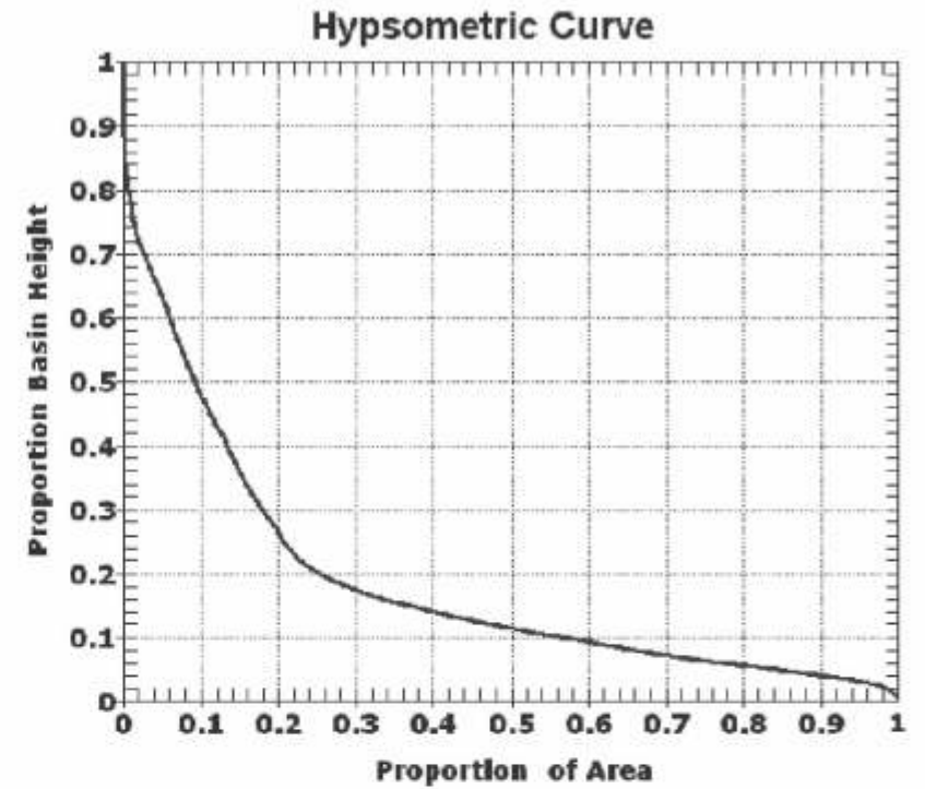
Figure 6 Hypsometric Curve
