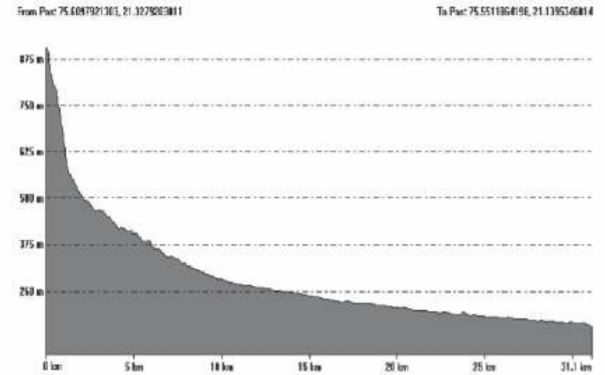
Figure 7 River longitudinal Profile
